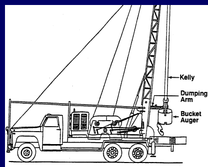
Setup of rig for bucket auger boring (ASTM D 4700)
